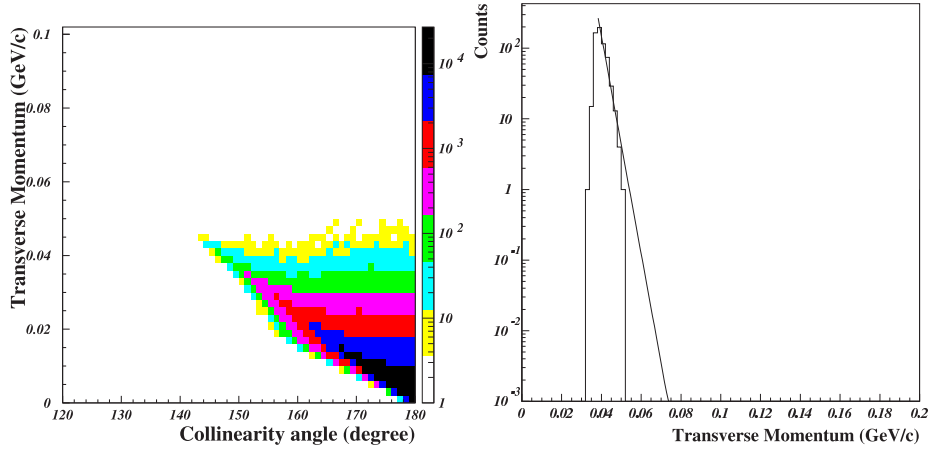
Figure 38: Monte Carlo study for the K_L \rightarrow \gamma\gamma decays. Left: Distribution of collinearity angle vs. P_T . Right: P_T distribution. The total number of generated events is equivalent to 9.7 \times 10^{10} of the K_L 's entering the detector setup, which is 0.05% of the total number of K_L 's in Step 1.
