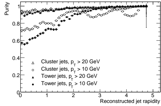
Figure 10.79: Purity of jet reconstruction in VBF-produced Higgs-boson events as a function of the rapidity y of the reconstructed jet for p_T^{\text{jet}} > 10 \text{ GeV} and p_T^{\text{jet}} > 20 \text{ GeV} and for cone-tower and cone-cluster jets with \Delta R = 0.7 .
