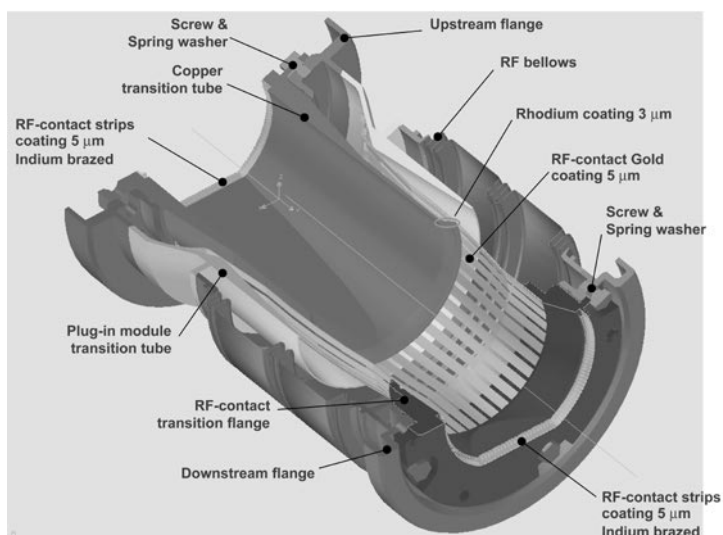
Figure 5.3: Details of the interconnect “plug-in module”.
