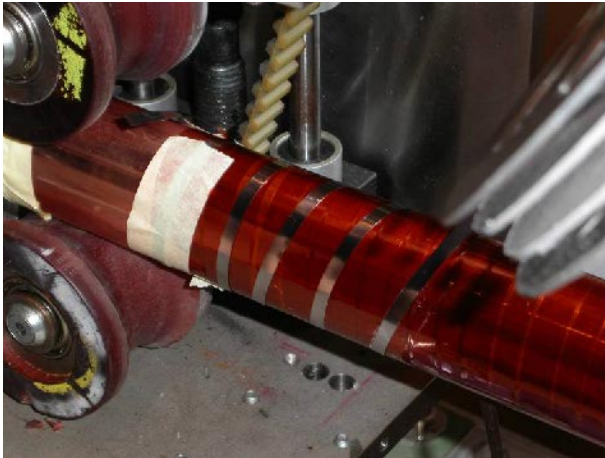
Figure 5.6: Wrapping of the stainless steel strips as bakeout heaters and a close up view of a finished chamber before the addition of the aluminised layer.
