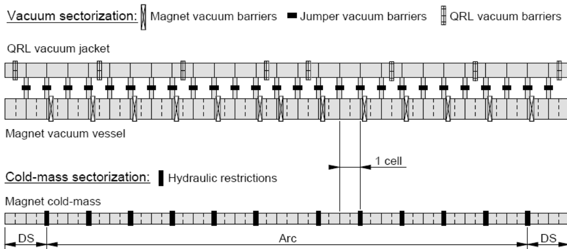
Figure 7.6: Cold-mass and cryogenic vacuum sub-sectorisation.
